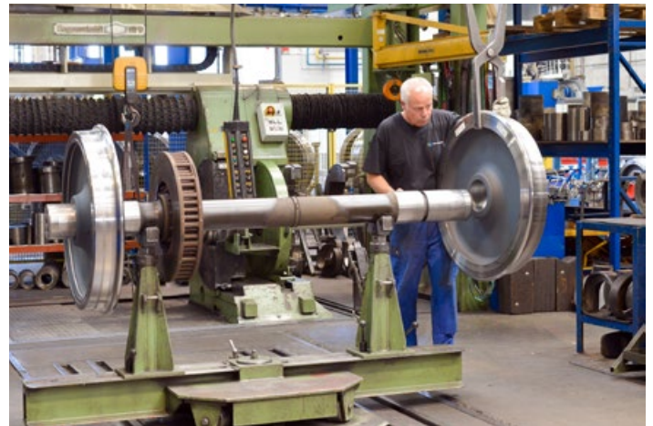
Overhaul of wheelsets
