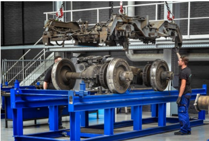
Handling of bogies
